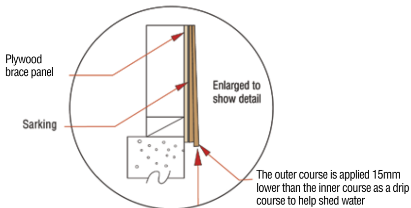
Figure 5: Single Coursing
