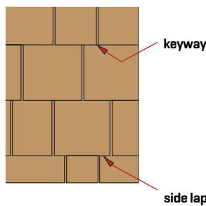
Figure 1: Spacing Detail
