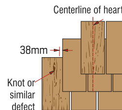
Figure 4: Course Alignment
