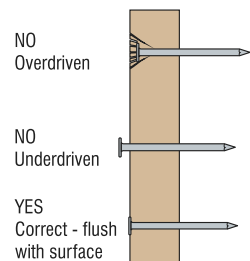
Figure 3: Nail Driving detail
