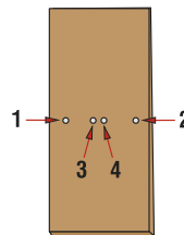
Figure 2: Wide Shingle Fastener detail
